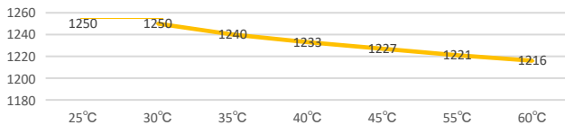
Temperature (CePEMius) Derate Curves Unit: kVA
