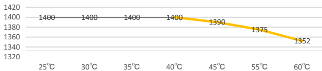
Temperature (CePEMius) Derate Curves Unit: kVA
